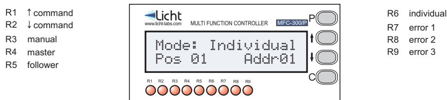
Figure 3.1 Front Panel
