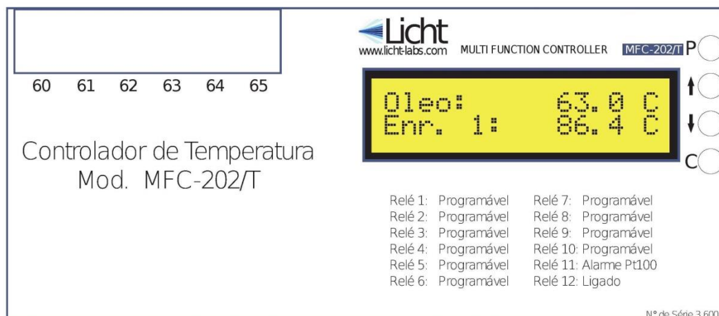
Figura 4.1. Painel Frontal
